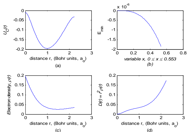
Figure 3 Z = 1, Hydrogen (H) , Yukawa potential
