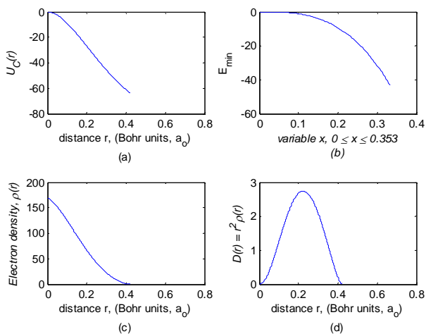
Figure 4 Z = 90, (Th) Yukawa potential
