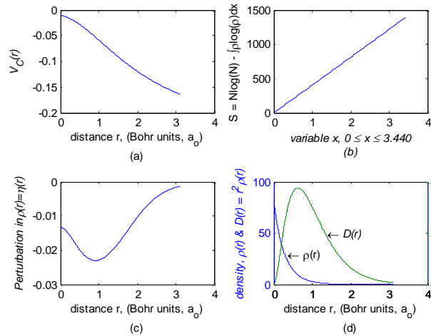
Figure 8 Z = 90 (Th) Perturbed, Yukawa.
