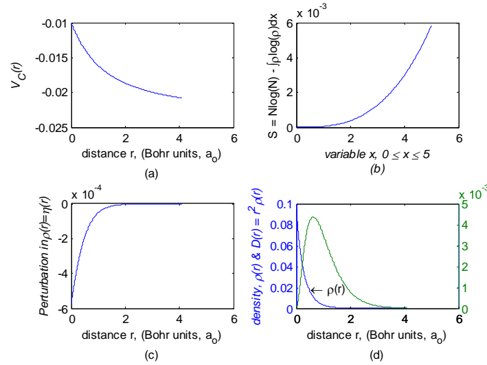
Figure 7 Z = 1 (H) Perturbed, Yukawa.
