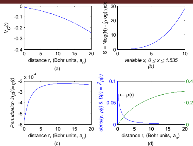
Figure 5 Z = 1, (H) perturbed Coulomb
