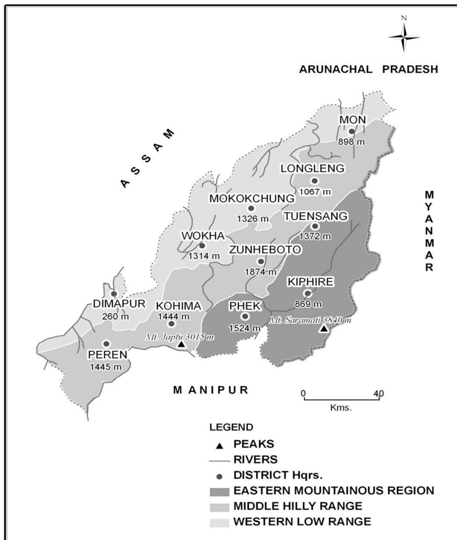
Fig.- 2 : Physiographic Map of Nagaland, India.
